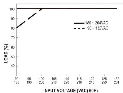
■Static characteristic
