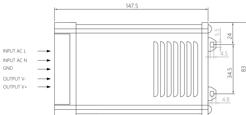
■Vertical view
