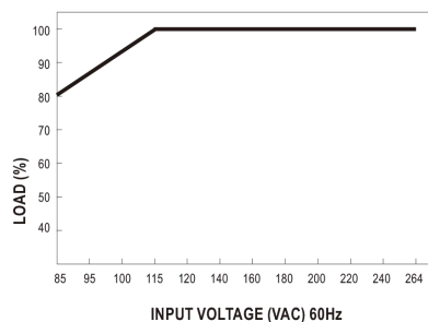
■Static characteristic
