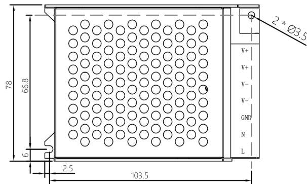
■Vertical view
