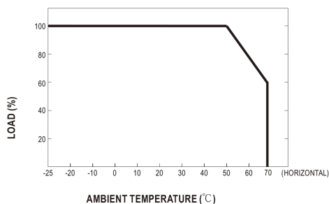
■Drating Curve
