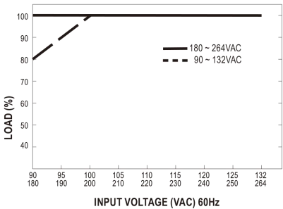
Static characteristic
