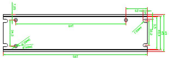
■Vertical view
